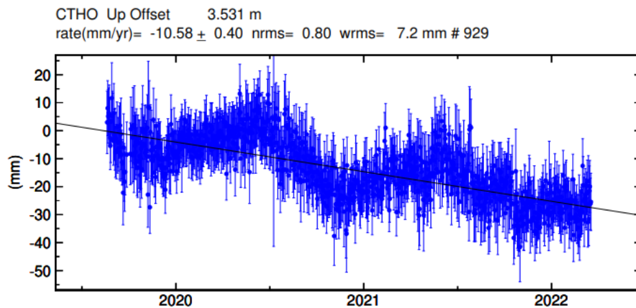
Figure 8. Graph of Up-component of CTHO CORS station determined by Gamit/Globk.
